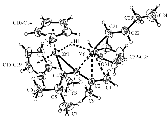
Figure 1. Molecular structure of the heterobimetallic Zr/Mg complex 5 . [17] Ellipsoids are set at 30% probability.
